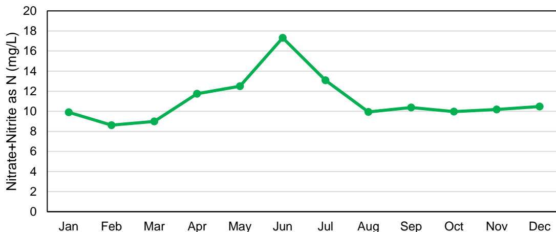
Figure 3.2.1. Monthly average nitrogen levels for samples collected from Howard Creek at Farmersburg from 1993 through 1998.
