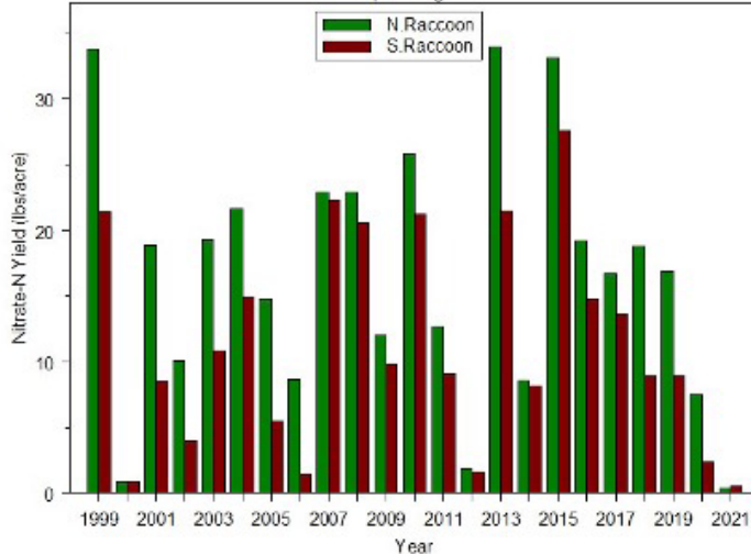
Raccoon River Nitrate Yield April - August
