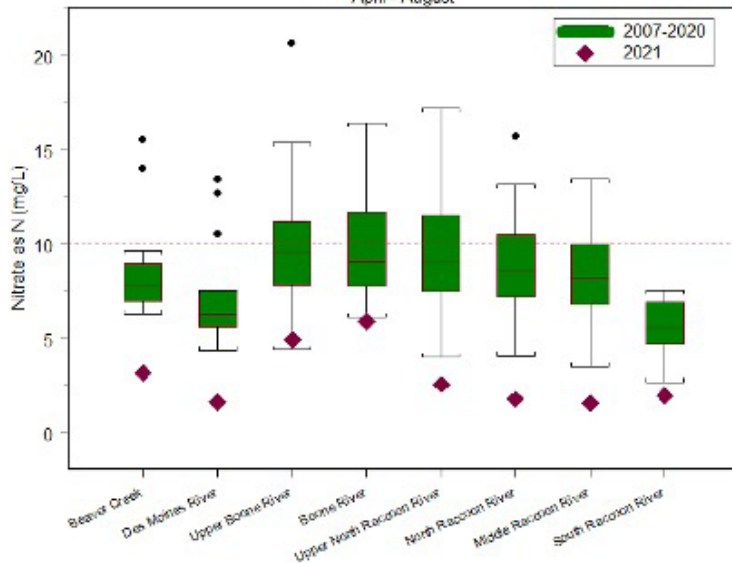
Average nitrate-N concentrations for major basins in the Raccoon and Des Moines River watersheds for 2007-2020 (range shown with boxplots) and 2021 (dots).
